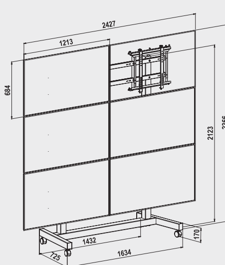
MOVYALL-H 3X2 cod. 08005 Single Side cod. 08007 BackToBack
