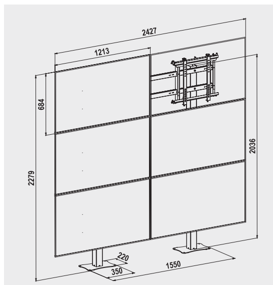
STANDYALL-H 3X2 cod. 08015 Single Side cod. 08018 Back to Back
