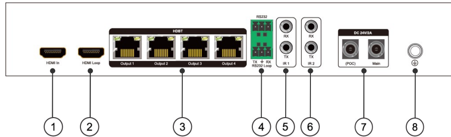
Rear Panel
