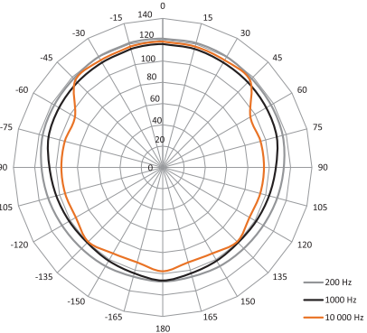
SAM-8 - NOMINAL VERTICAL COVERAGE
