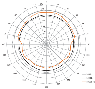
SAM-5 - NOMINAL HORIZONTAL COVERAGE
