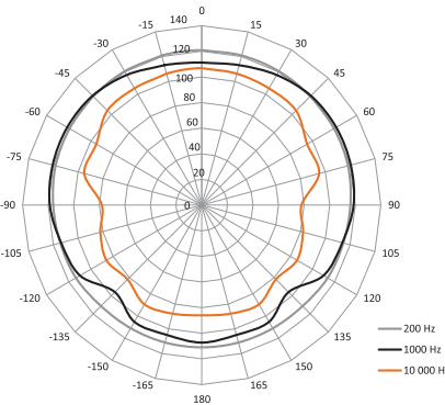
SAM-12 - NOMINAL VERTICAL COVERAGE
