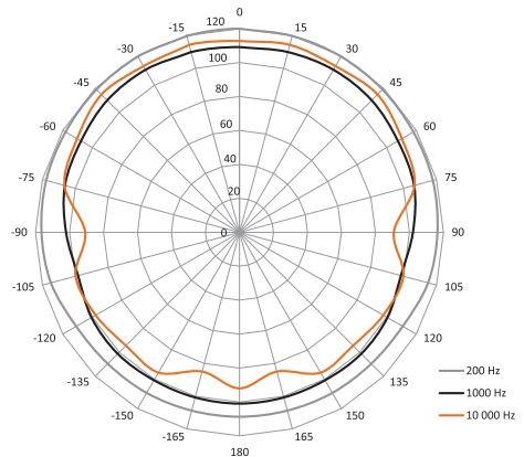
SAM-15 - NOMINAL VERTICAL COVERAGE
