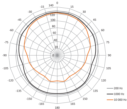
SAM-12 - NOMINAL HORIZONTAL COVERAGE
