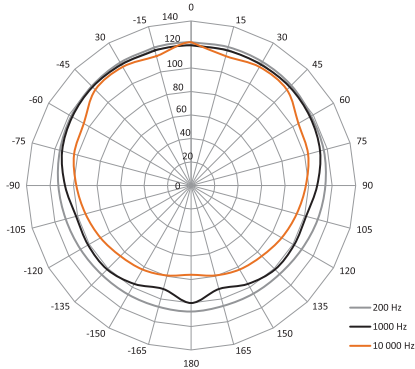
SAM-8 - NOMINAL HORIZONTAL COVERAGE
