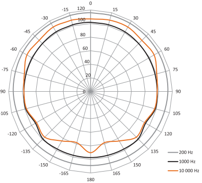
SAM-5 - NOMINAL VERTICAL COVERAGE
