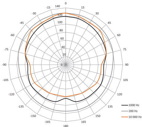
SAM-15 - NOMINAL HORIZONTAL COVERAGE
